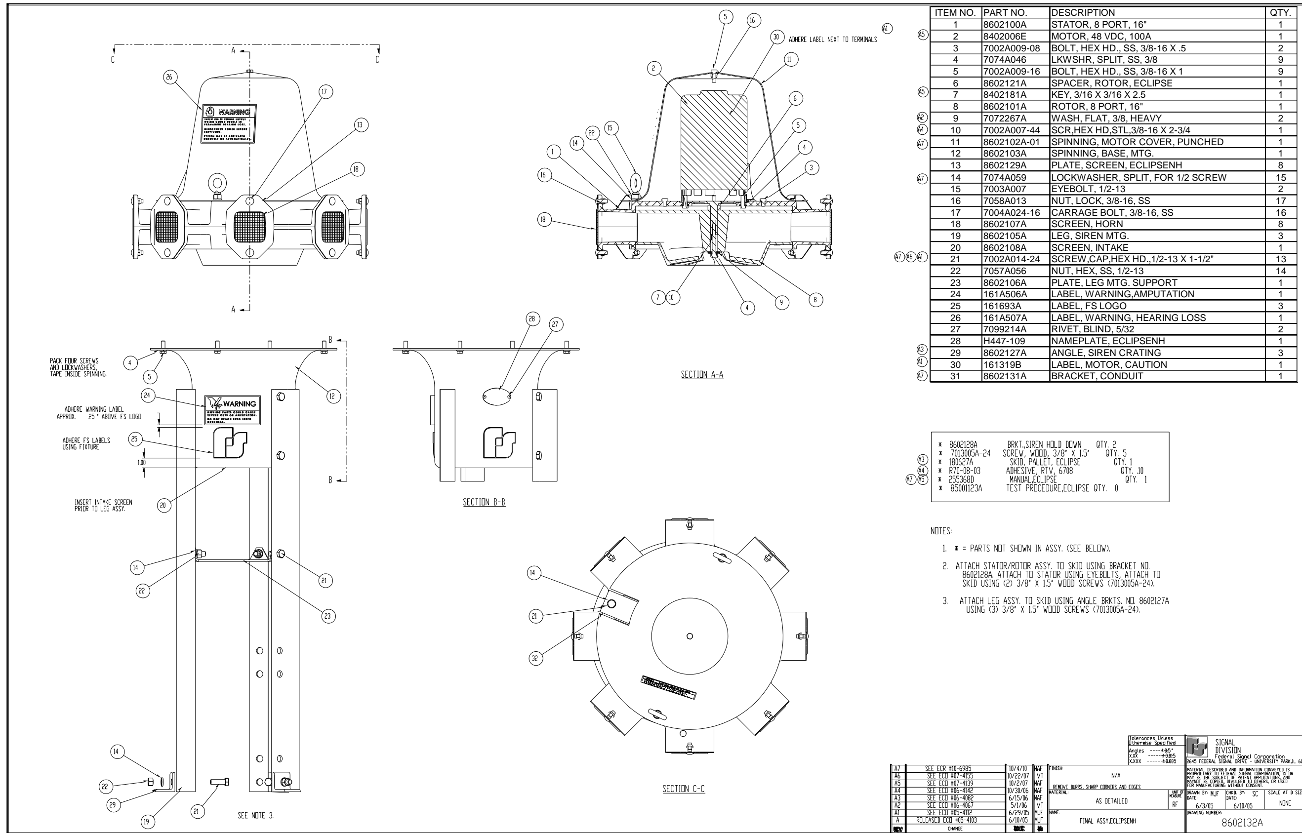
Figure 4-2 EclipseNH Parts List
